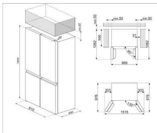
FQI60KD
