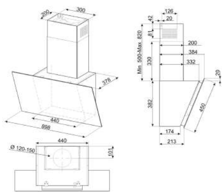
KICV90BL
