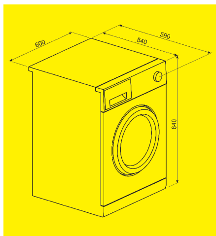
LB2T82ASIT
