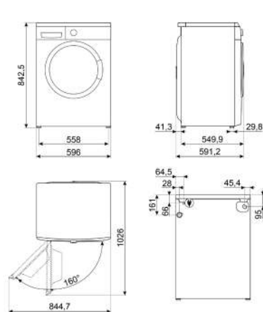
LB1T80IT
