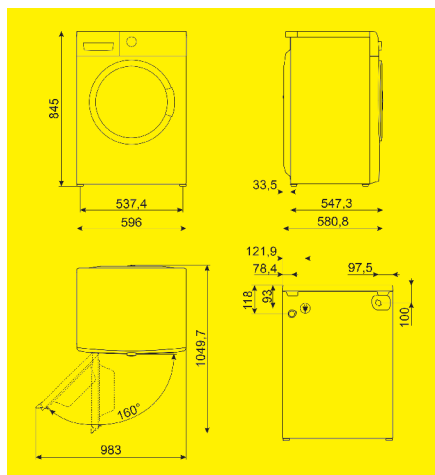
LB2T02ASIT
