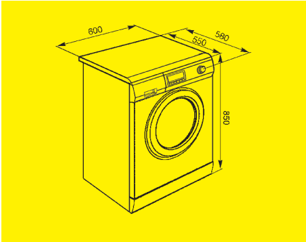
WNG24SLAA10
