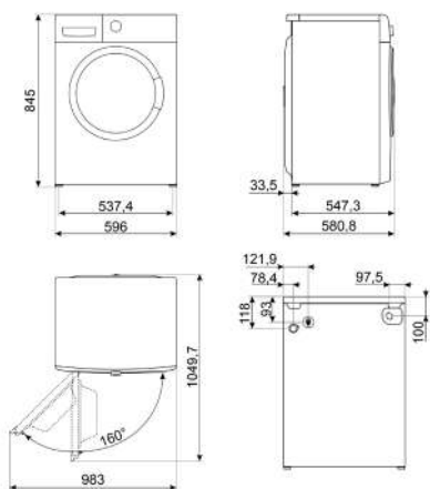
WN04SEA, WN94SEA, WN84SEA
