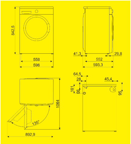
WNG94SEA10
