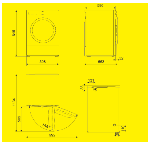
DN03SE
