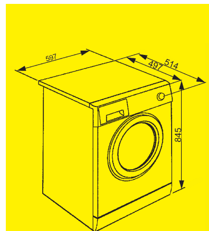
LB2T92ASIT
