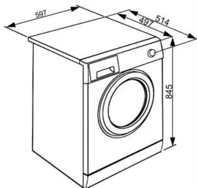
LBW60IT
