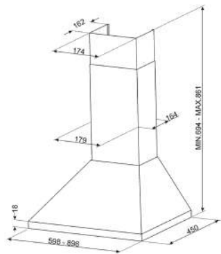
KDE900EX, KDE600EX
