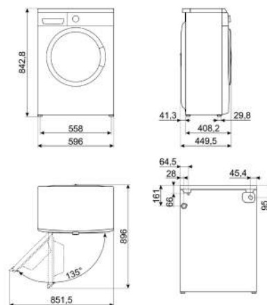
LBW62PCIT
