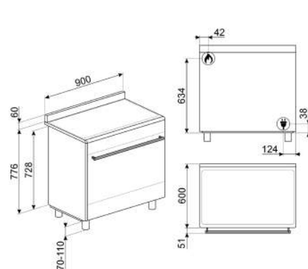
SX91GM
